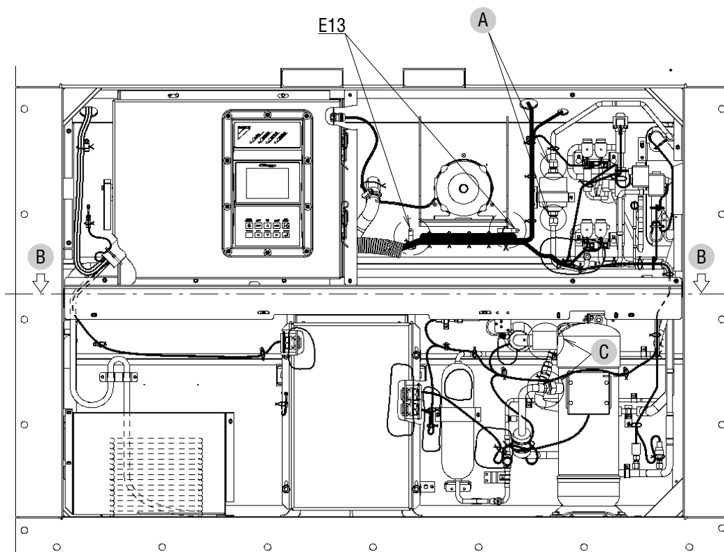
A詳細(Detail of A)
