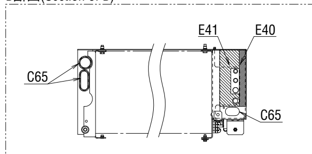
B断面(Section of B)
