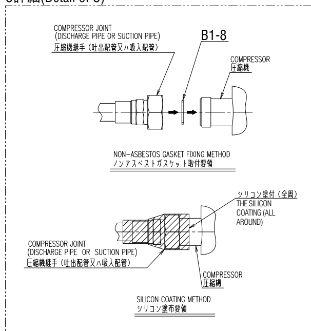
C詳細(Detail of C)
